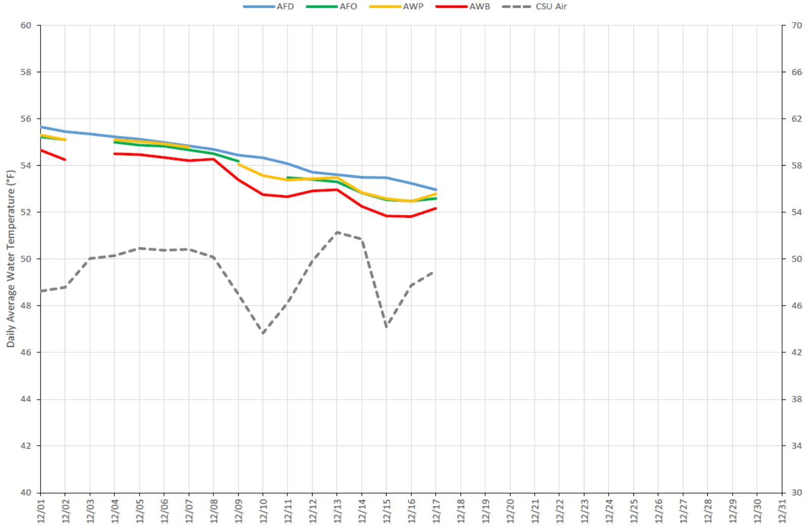
American River Daily Average Water and Air Temperatures (Calendar Year 2024)
